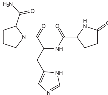
TRH (Thyrotropin-releasing hormone), Protirelin
