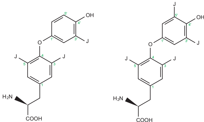
3,5,3'-Trijod-L-thyronin, T_3 , Liothyronin
