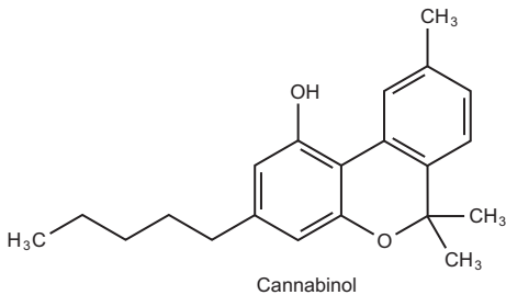
Cannabinol
