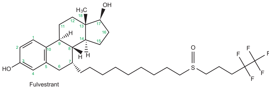
Fulvestrant
