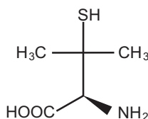
Penicillamin
