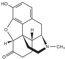
Hydromorphon
