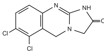
Anagrelid
