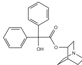
3-Chinuclidinylbenzilat, BZ
