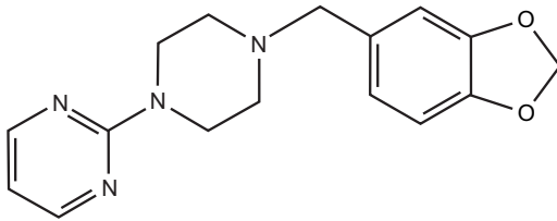
Piribedil
