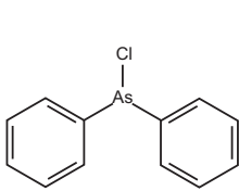
Clark 1, DA Diphenylchlorarsin
