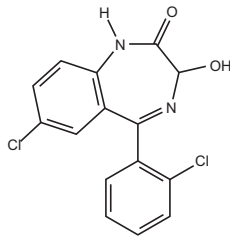
Lorazepam
