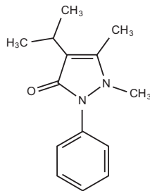
Propyphenazon
