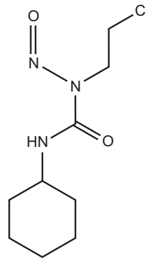
Lomustin
