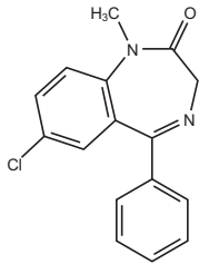
Diazepam
