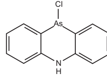
Adamsit, DM Diphenylaminchlorarsin
