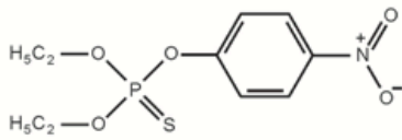
Parathion (Pestizid)
