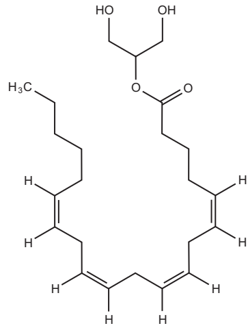
2-Arachidonylglycerol
