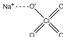
Natriumperchlorat
