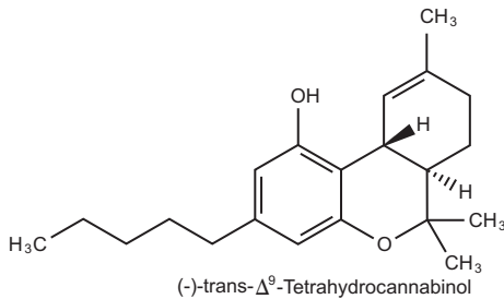
(-)-trans- \Delta^9 -Tetrahydrocannabinol
