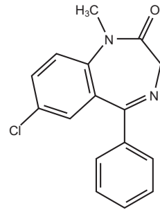
Diazepam
