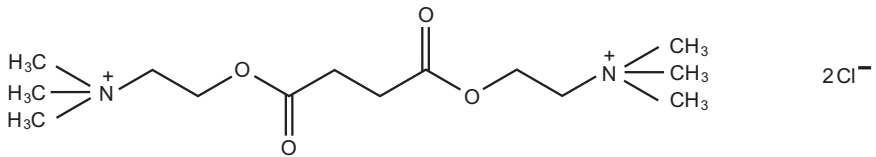
Suxamethonium-Dichlorid, Succinylcholin
