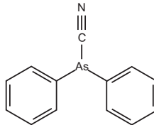
Clark 2, DC Diphenylcyanarsin
